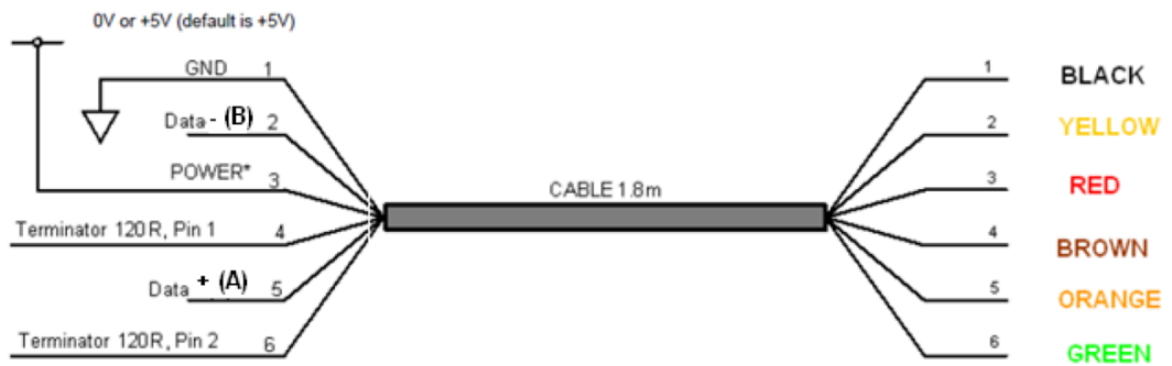
Figure 5.1 USB-RS485-WE Connections
